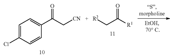
Scheme 1. Synthesis of compounds of Formula I wherein R 4 = D 9 -t-butyl
