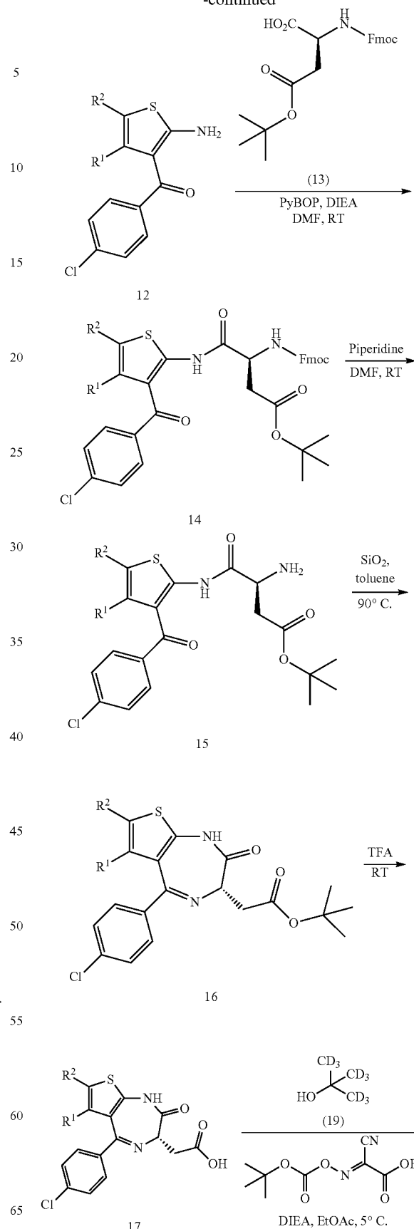
Scheme 1. Synthesis of compounds of Formula I wherein R 4 = D 9 -t-butyl
