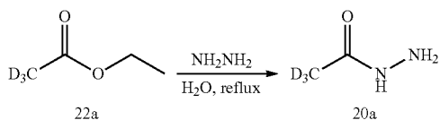
Scheme 4. Synthesis of 20a
