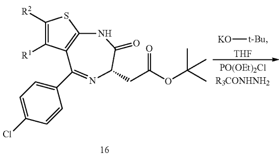
Scheme 2. Synthesis of compounds of Formula I wherein R^4 = \text{---C}(\text{CH}_3)_3 .
