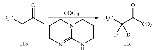
Scheme 3. Synthesis of 11c
