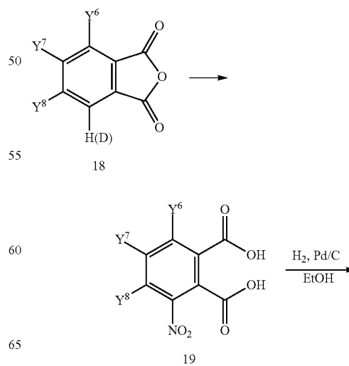
Scheme 3. Preparation of intermediates 12a and 12b.
