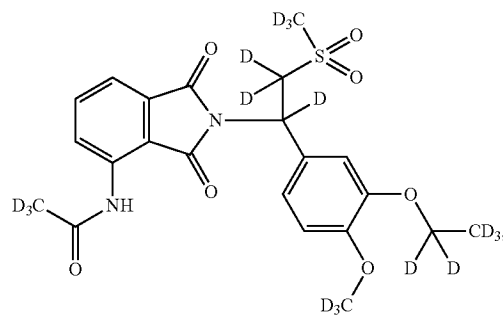
Compound 102
