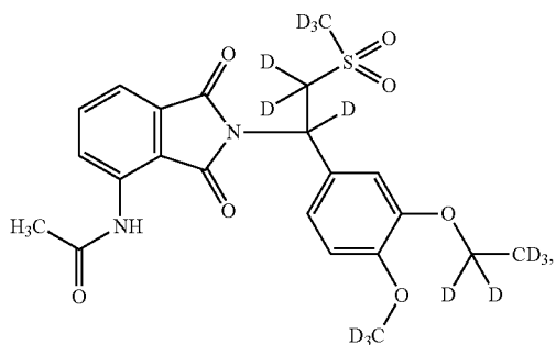
Compound 104
