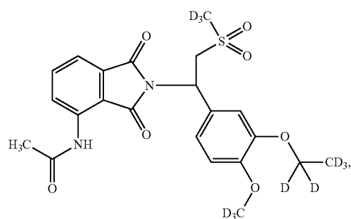
Compound 106
