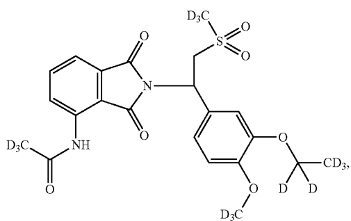
Compound 103
