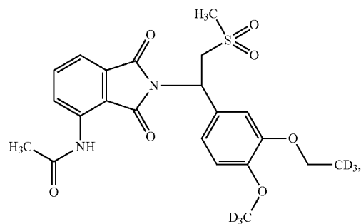
Compound 109
