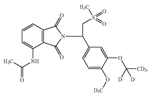
Compound 107
