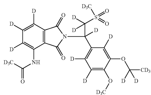
Compound 101
