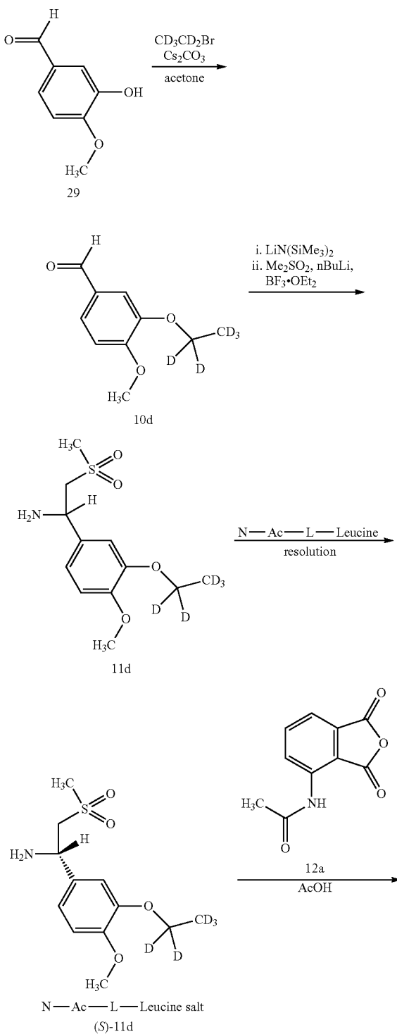
Scheme 7. Preparation of Compound 110a.
