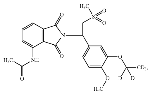
Compound 110
