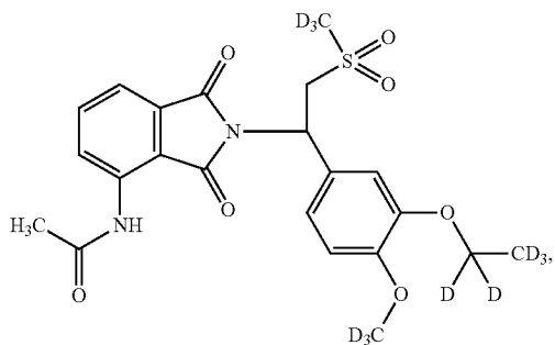
Compound 106
