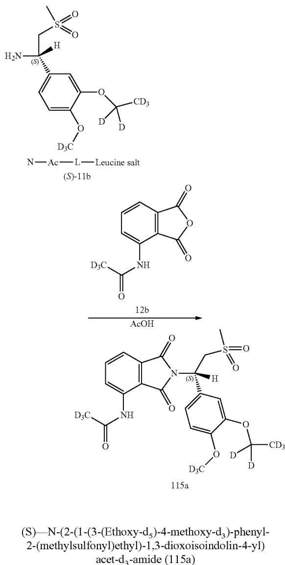
Scheme 8. Preparation of 115a.
