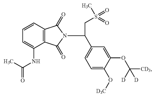
Compound 107
