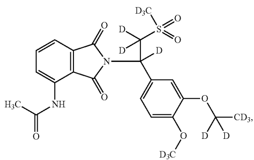
Compound 104
