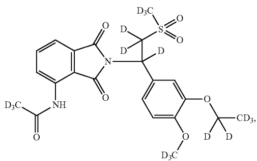
Compound 101
