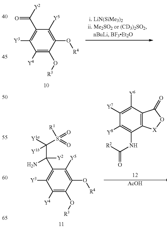
Scheme 1: General Route to Compounds of Formula I.
