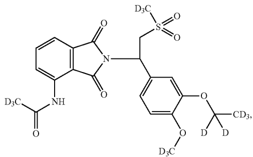
Compound 103
