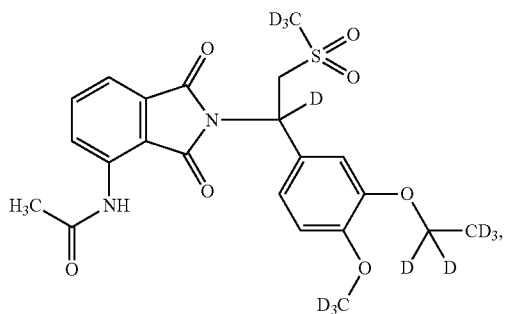
Compound 105
