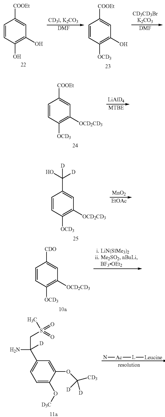
Scheme 4. Preparation of Compound 113a.
