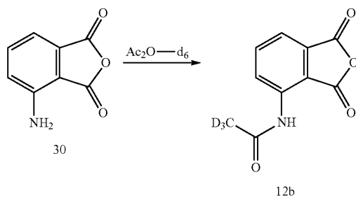
Scheme 8. Preparation of 12b.
