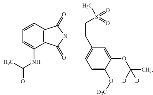
Compound 108
