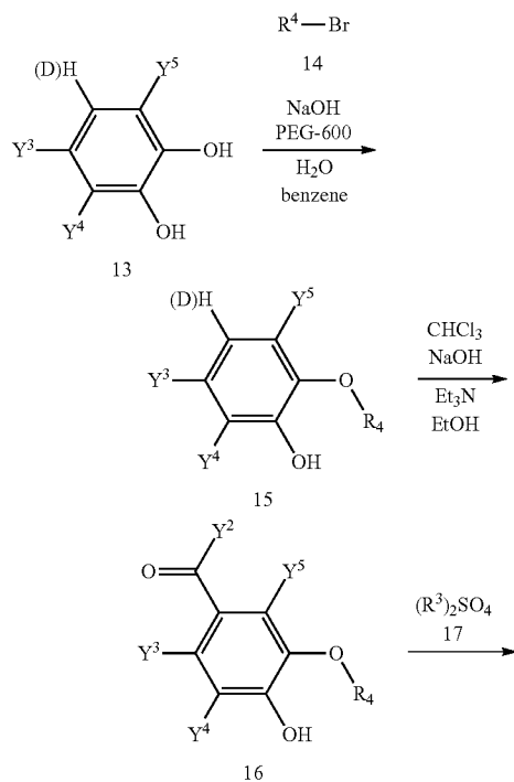
Scheme 2: Preparation of aldehyde 10.
