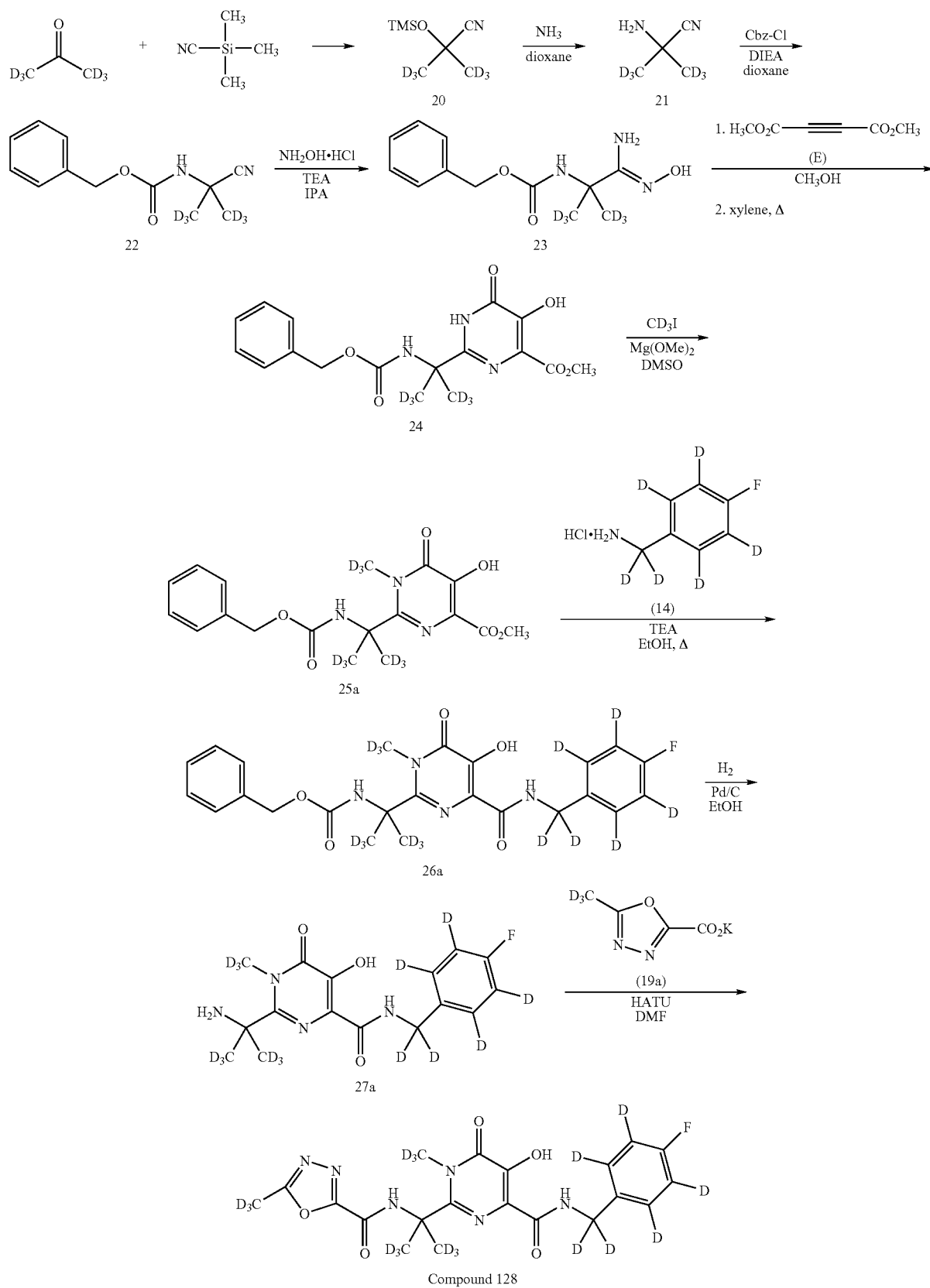
Compound 128
