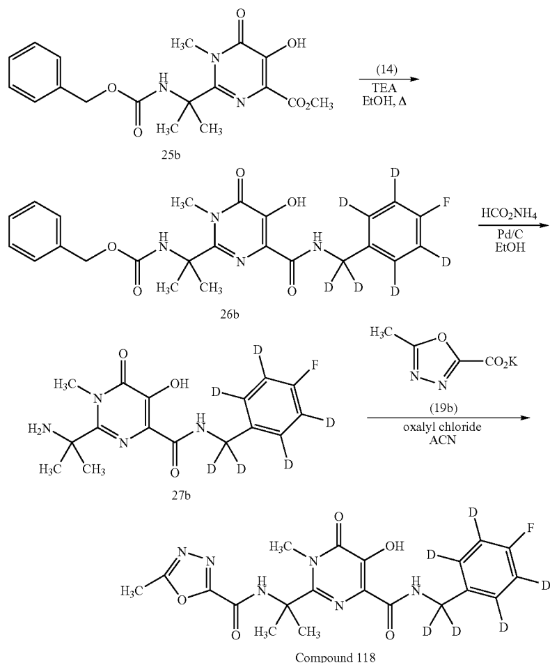
Scheme 7
