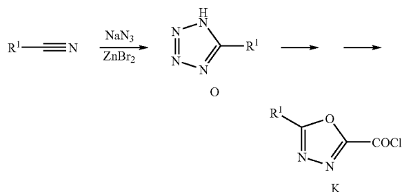
Scheme 3. Synthesis of Compound K.
